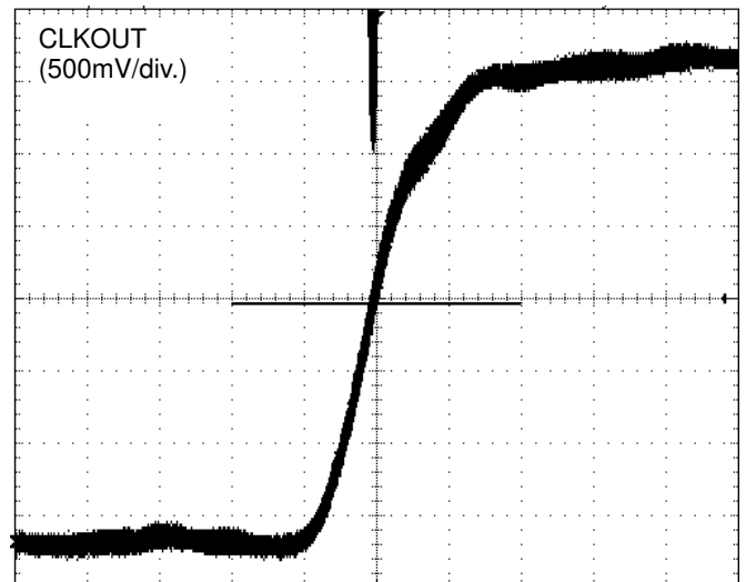
Figure 8. CLKOUT Period-Jitter
