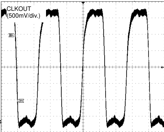
Figure 7. CLKOUT Output Waveform
