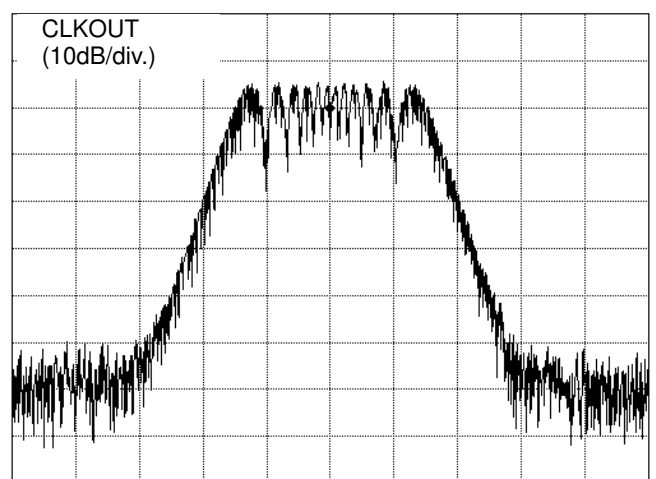
Figure 28. CLKOUT±1.00% Modulation Spectrum
