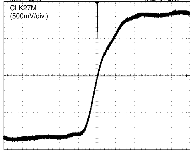
Figure 6. CLK27M Period-Jitter
