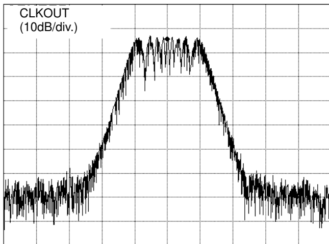
Figure 27. CLKOUT±0.75% Modulation Spectrum
