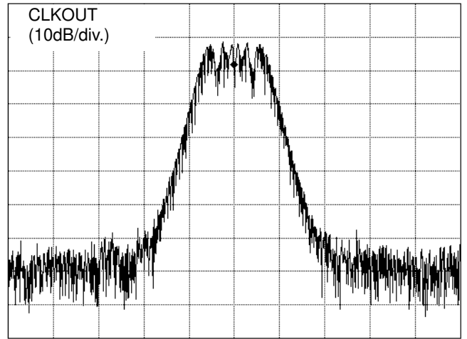
Figure 26. CLKOUT±0.50% Modulation Spectrum
