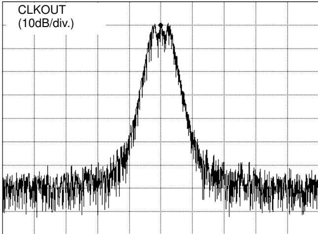
Figure 25. CLKOUT±0.25% Modulation Spectrum
