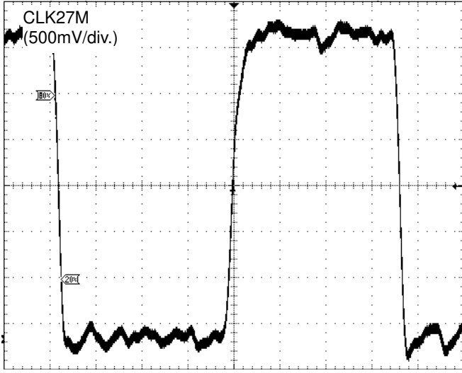
Figure 5. CLK27M Output Waveform
