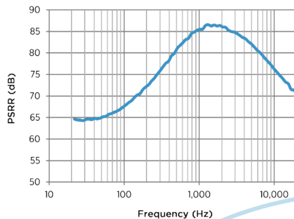
Figure 9: Typical PSRR
