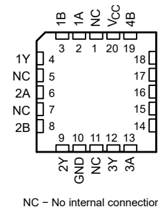
Figure 5-4. SN54AHC86 FK Package, LCCC 20-Pin (Top View)
