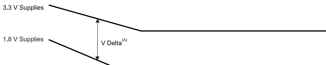
Figure 8-3. 1.8 V Supplies Falling Before 3.3 V Supplies Delta
