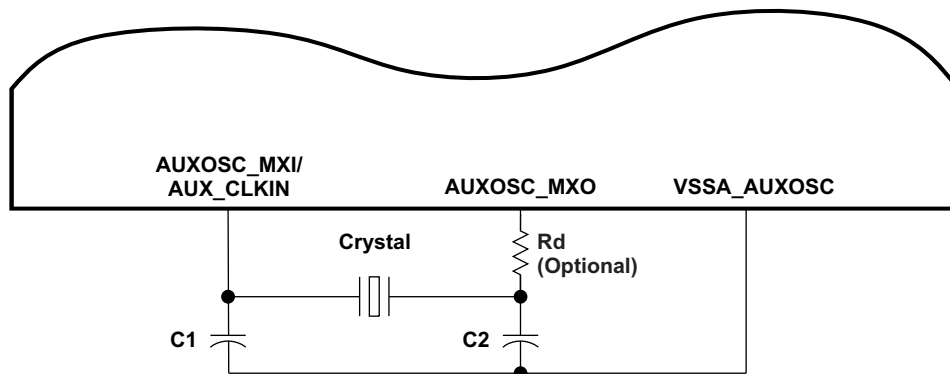
Figure 8-8. Auxiliary Oscillator
