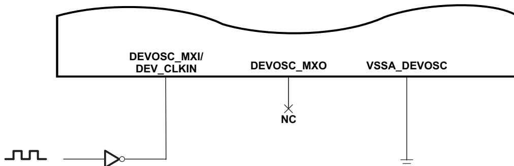
Figure 8-9. 1.8-V LVCMOS-Compatible Clock Input (DEV_OSC)
