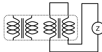
Differential Mode
