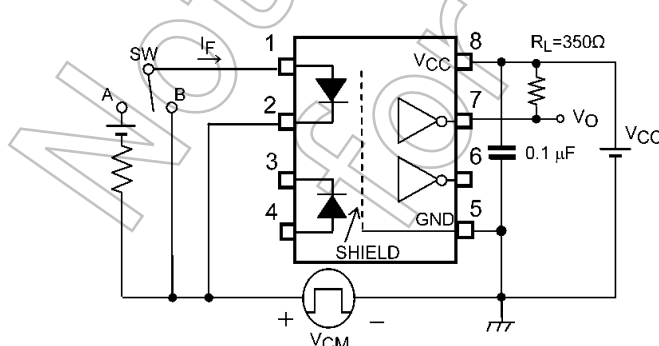
Fig. 12.1.6 Common-Mode Transient Immunity and Waveform
