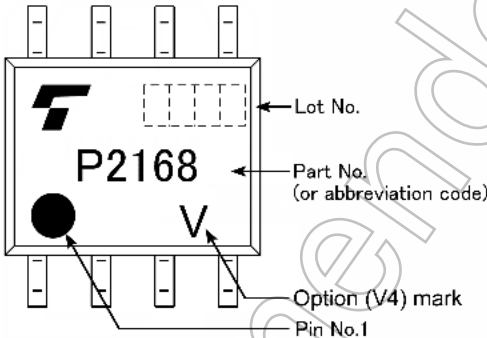
Fig. 16.3 Marking Example(Note 1)
