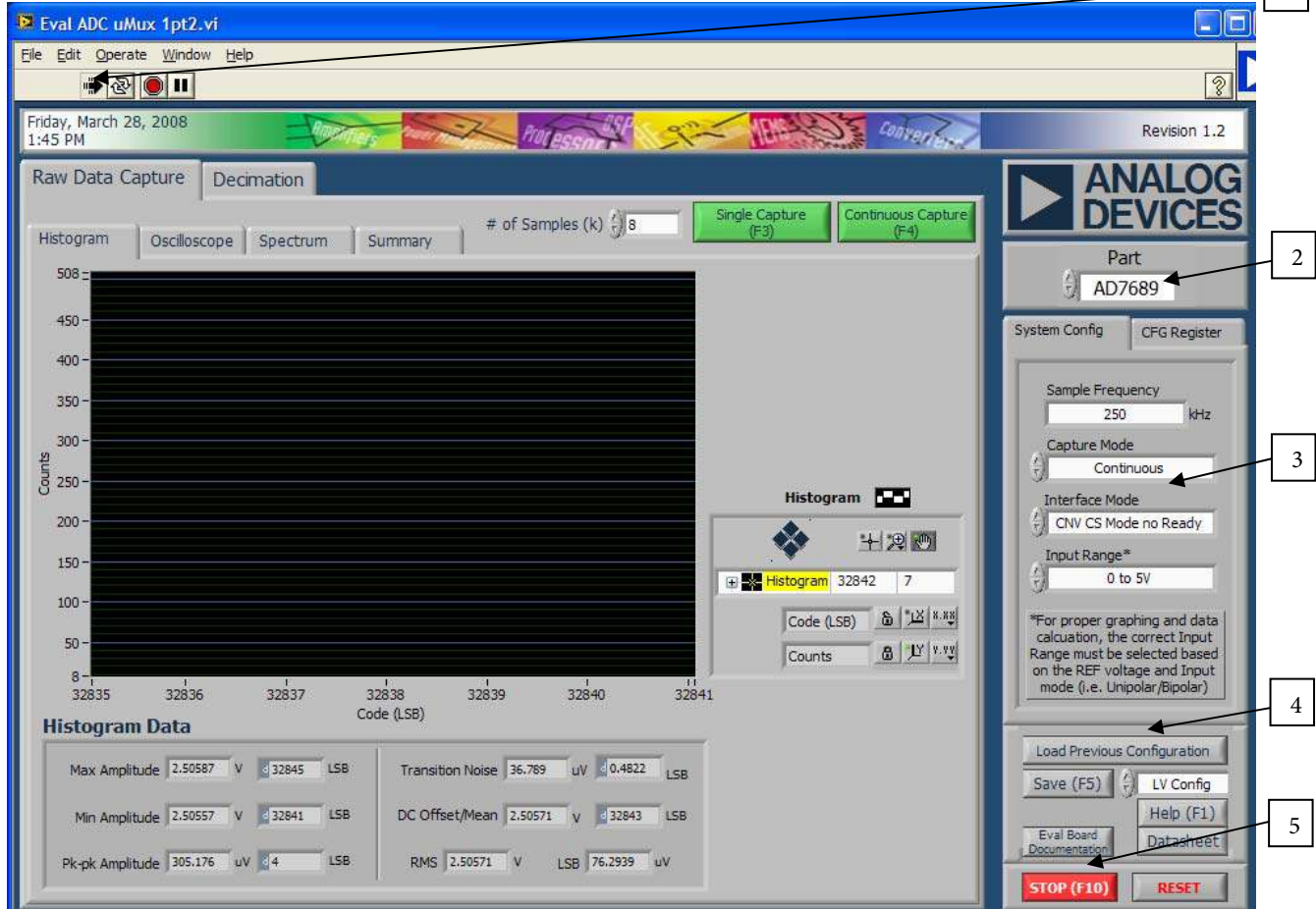
Figure 2. Setup Screen
