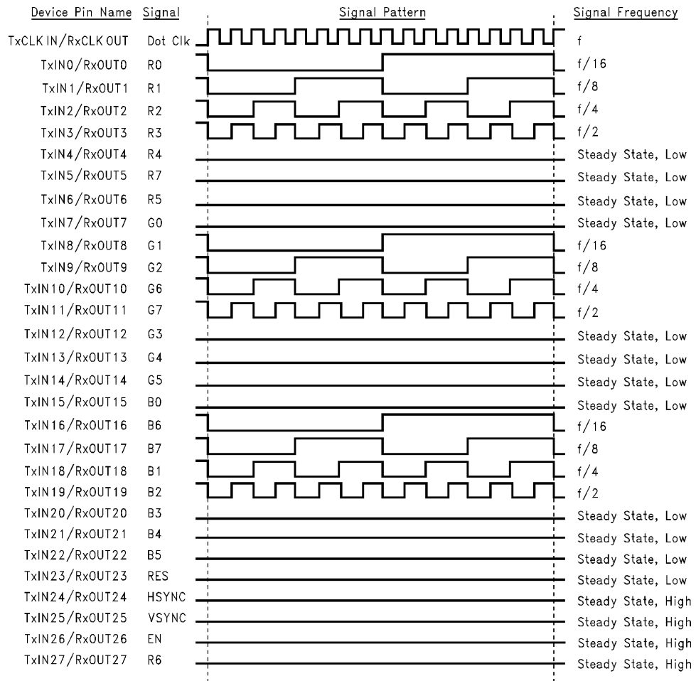
FIGURE 2. "16 Grayscale" Test Pattern (Notes 7, 8, 9, 10)
