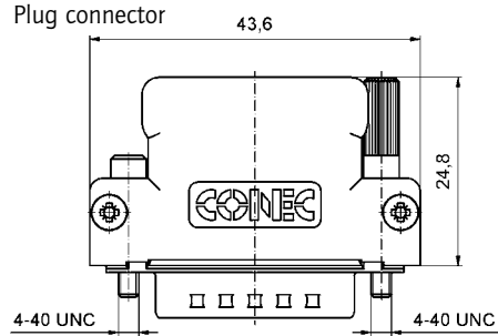
Plug connector
