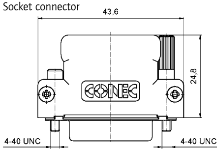
Socket connector
