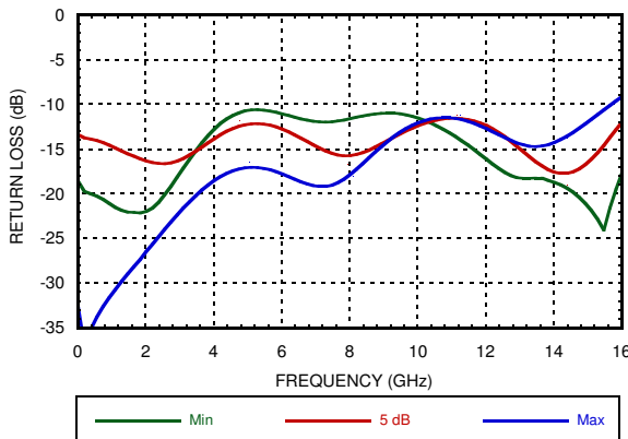
Return Loss vs. Attenuation
