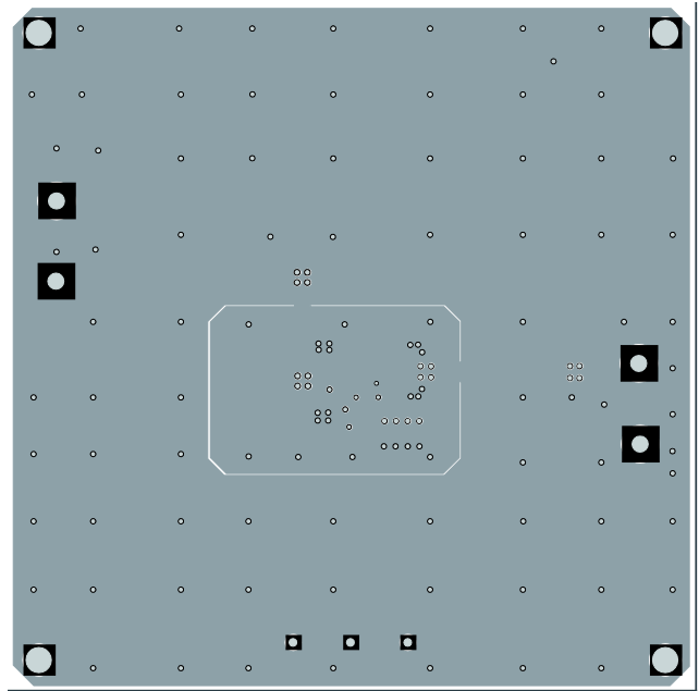
Figure 3: Inner1 Layer
