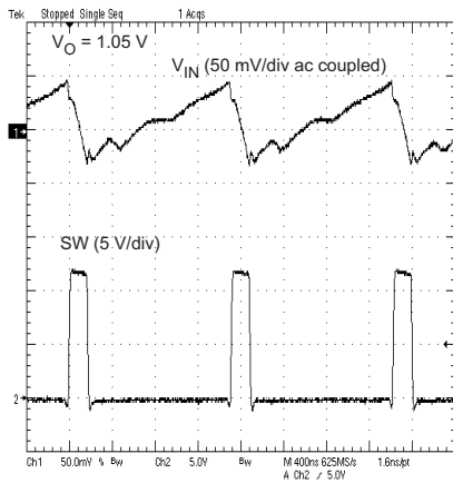
Figure 8-10. Voltage Ripple at Input ( I_O = 5.5\text{ A} )
