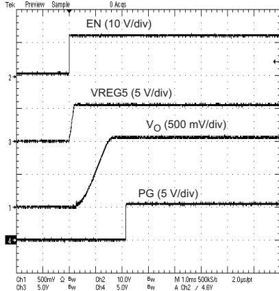
Figure 6-7. Start-Up Waveform
