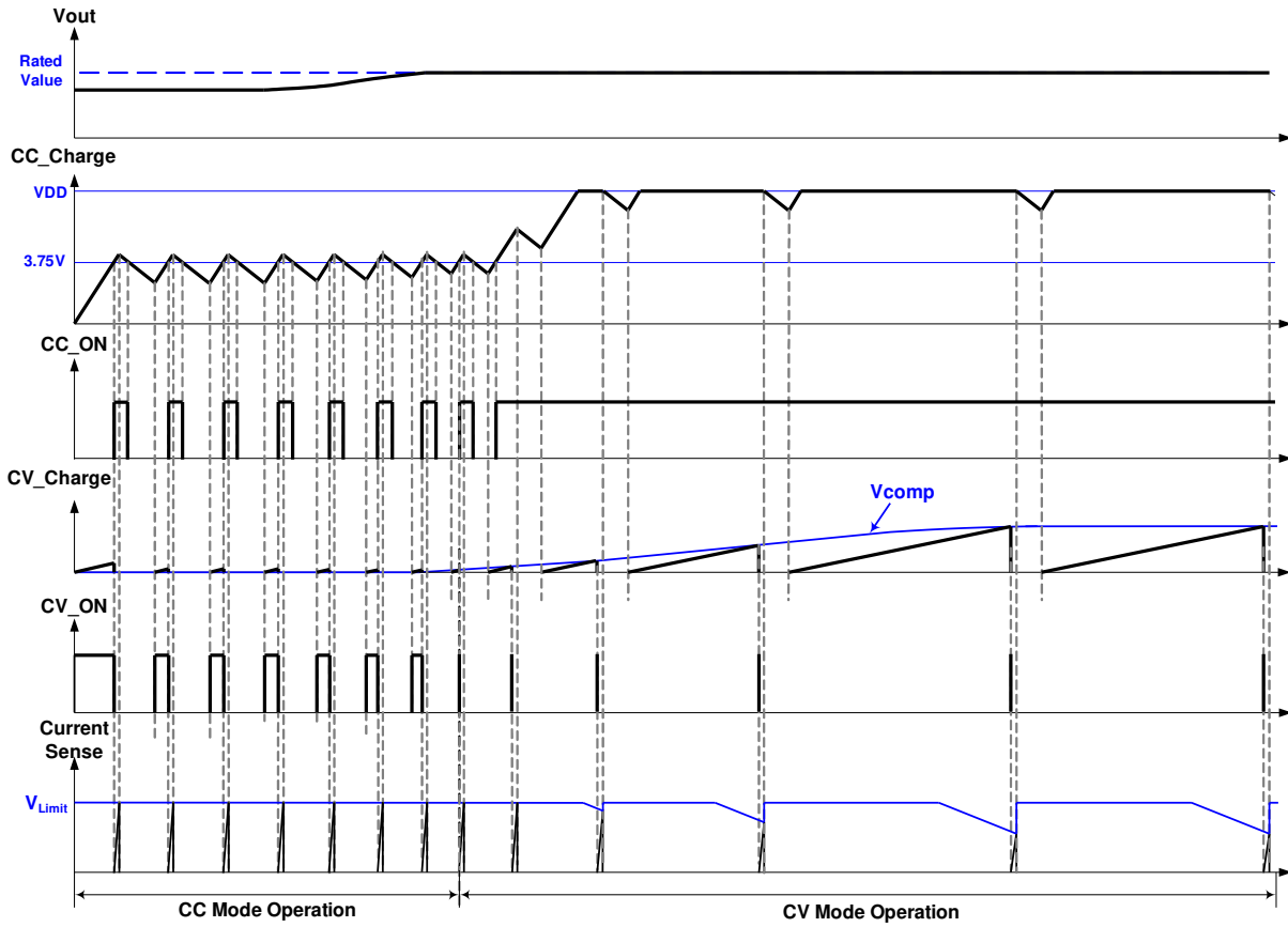
Figure 18: Start-Up Sequence
