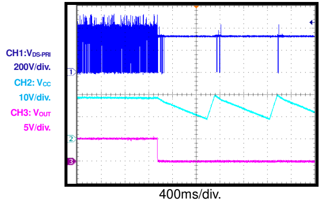
Short-Circuit Entry
