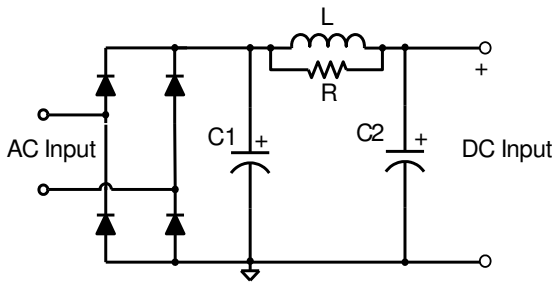
Figure 10: Input Filter
