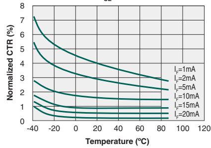
Typical Normalized CTR vs. Temperature (V CE =0.5V)
