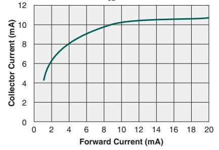
Typical Collector Current vs. Forward Current (V CE =0.5V)
