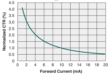
Typical Normalized CTR vs. Forward Current (V CE =0.5V)
