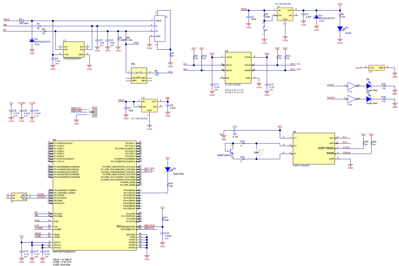
Figure 4-1. TMP451EVM Schematic
