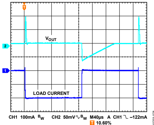
Figure 80. Output Transient Response, C_{\text{out}} = 2.2 \mu\text{F}
