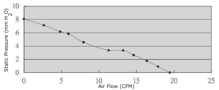
CFM-5015BF-175-423
