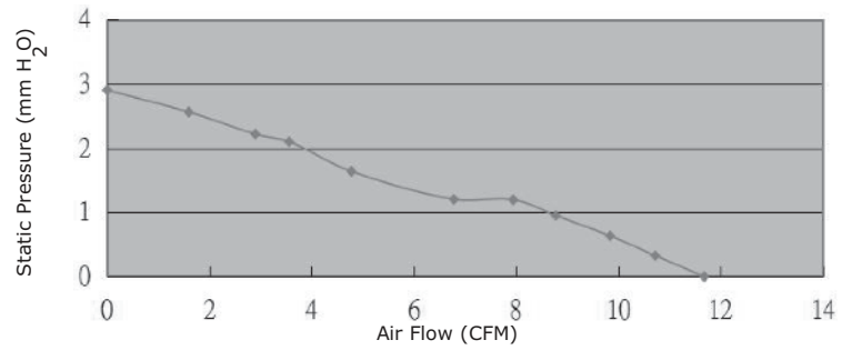
CFM-5015BF-145-312
