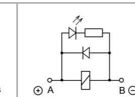
C: Option 6, 7, 74 LED + diode (DC, polarity positive to pin A/A1)
