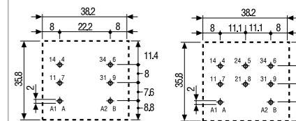
62.22 - 0300 Copper side view
