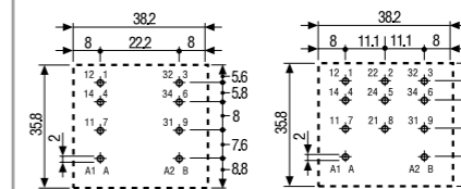
62.22 Copper side view
