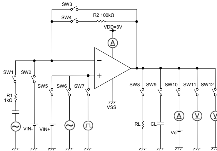
Figure 72. Test circuit 2
