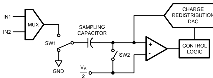
Figure 48. ADC122S051 in Hold Mode
