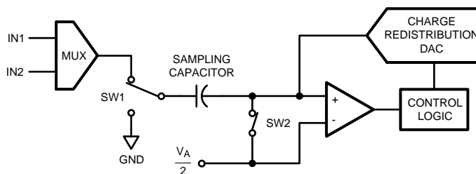
Figure 47. ADC122S051 in Track Mode
