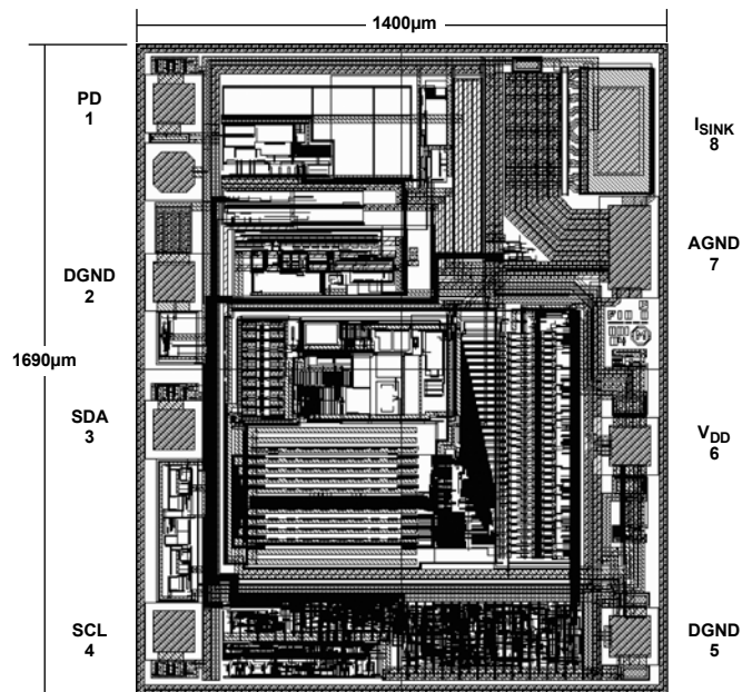
Figure 4. Metallization Photograph Dimensions shown in µm Contact Factory for Latest Dimensions
