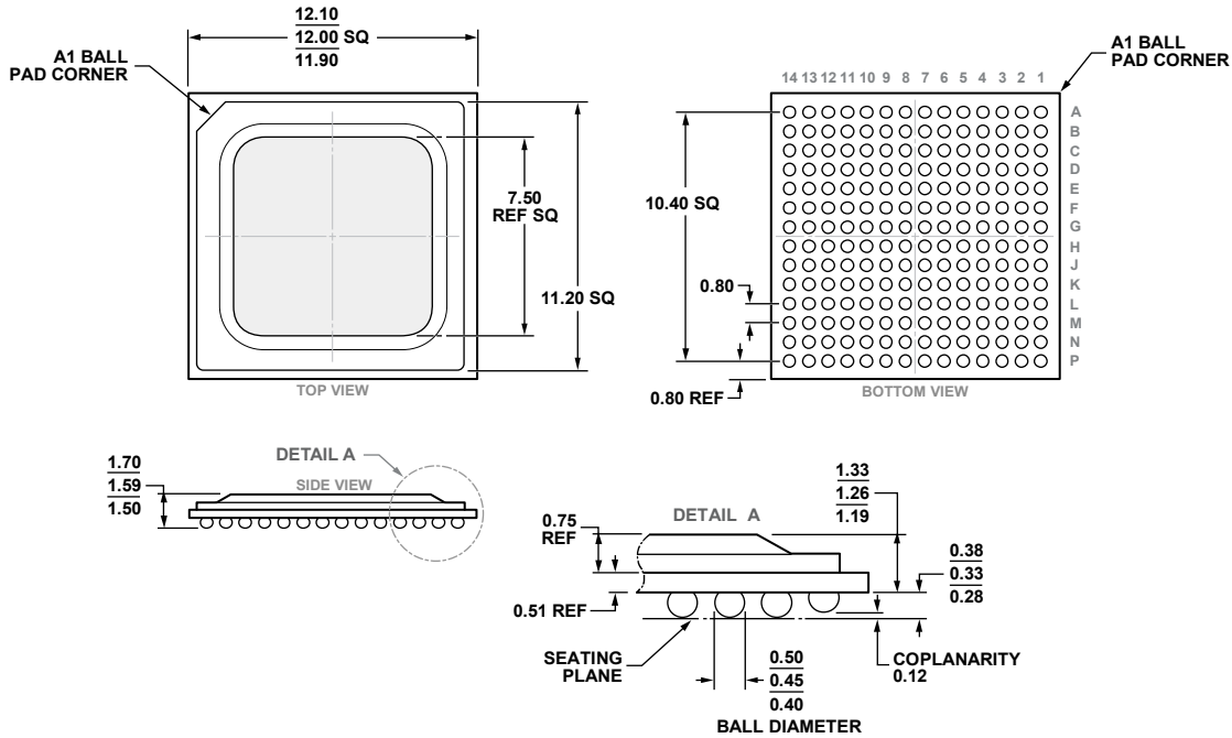
COMPLIANT TO JEDEC STANDARDS MO-275-GGAB-1. Figure 107. 196-Ball Ball Grid Array, Thermally Enhanced [BGA_ED] (BP-196-2) Dimensions shown in millimeters
