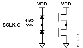
Figure 62. Equivalent SCLK Circuit
