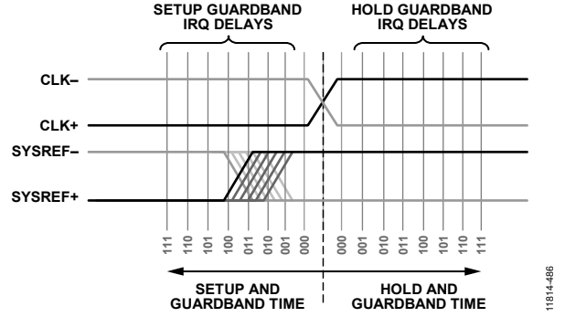
Figure 101. SYSREF\pm Edge Changes Phase Relative to the Encode Clock, Which can be Detected When the Edge Crosses Through the Guardband Setup Time
