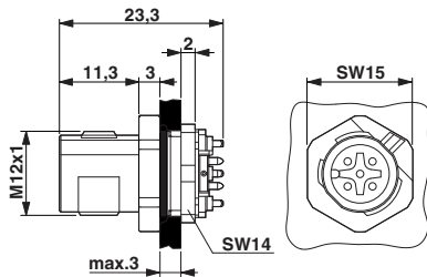
M12 flush-type plug
