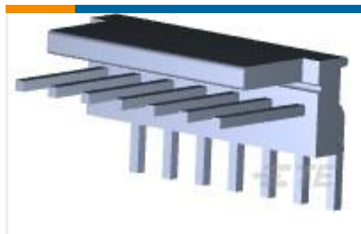
TE Part #640455-7 07P MTA100 HDR ASSY SQ R/A POL
