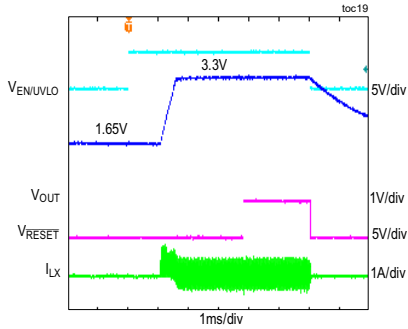
MAX17524, 3.3V OUTPUT SOFT-START WITH PREBIAS VOLTAGE OF 1.65V (PWM MODE, 0.66kΩ RESISTIVE LOAD, f_{sw} = 450kHz )
