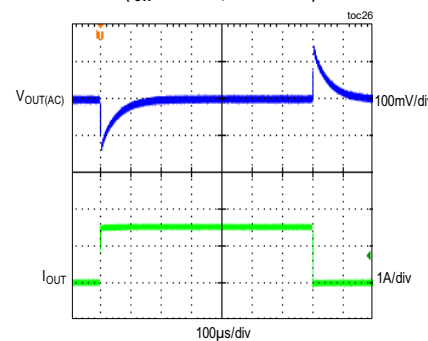
MAX17524, 5V OUTPUT LOAD TRANSIENT BETWEEN 0A AND 1.5A ( f_{sw} = 450kHz , PWM MODE)
