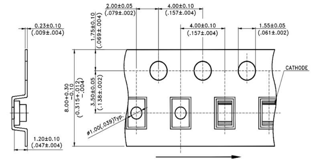
PACKAGE DIMENSION OF TAPE AND REEL
