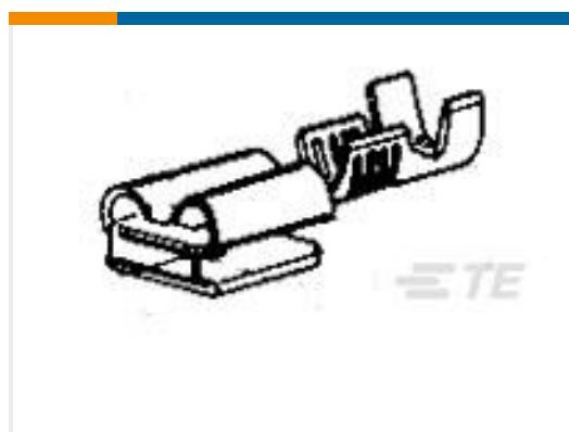
TE Part #150645-2 250 FASTON, REC., 18-14 AWG, BR
