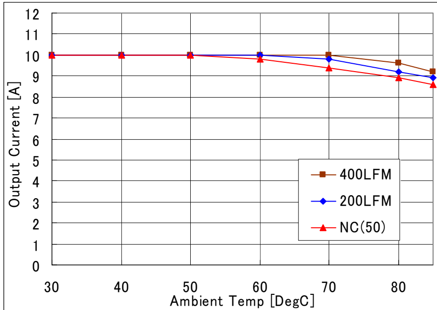
Fig-3.3V-1: Available load current vs. ambient temperature and airflow rates for Vout=3.3V with Vin=12.0V. Maximum component temperature \leq 120^{\circ}\text{C}
