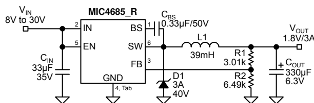
1.8V Output Converter
