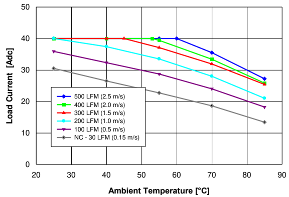
Fig. 2: Available load current vs. ambient air temperature and airflow rates for converter with G height pins mounted horizontally with air flowing from pin 1 to pin 3, MOSFET temperature \leq 120\text{ }^{\circ}\text{C} , V_{in} = 48\text{ V}
