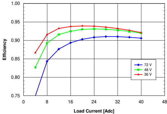
Fig. 3: Efficiency vs. load current and input voltage for converter mounted vertically with air flowing from pin 1 to pin 3 at a rate of 300 LFM (1.5 m/s) and T_a = 25\text{ }^{\circ}\text{C} .
