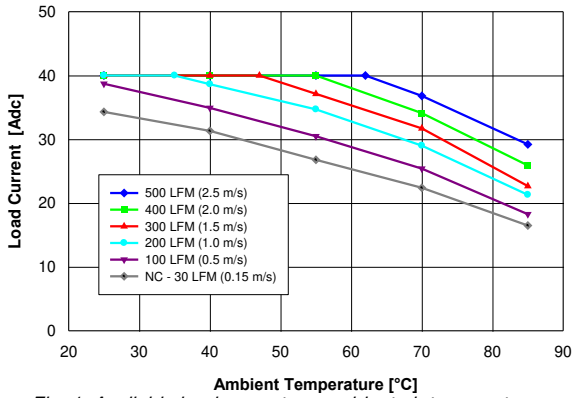
Fig. 1: Available load current vs. ambient air temperature and airflow rates for converter with G height pins mounted vertically with air flowing from pin 1 to pin 3, MOSFET temperature \leq 120\text{ }^{\circ}\text{C} , V_{in} = 48\text{ V} Note: NC – Natural convection
