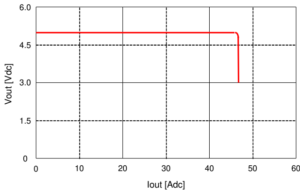
Fig. 15: Output voltage vs. load current showing load limit point and converter shutdown point. Input voltage has almost no effect on current limit characteristic
