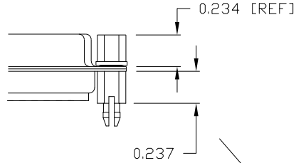
91 ..... 0.237" BOARD SIDE
