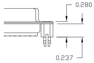
90 ..... 0.237" (BOARD SIDE)
