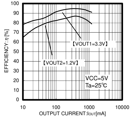
Fig.8 Efficiency
