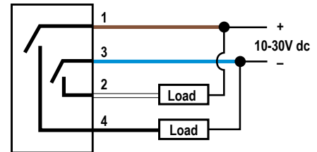
Figure 2. LS4R Receiver. Quick disconnect wiring diagrams are functionally identical.
