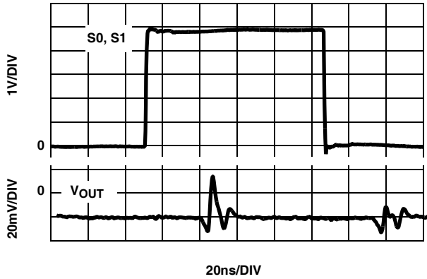
FIGURE 13. CHANNEL TO CHANNEL SWITCHING GLITCH V_{IN} = 0V , R_S = 25 , C_L = 23.6pF
