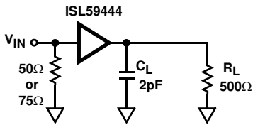
FIGURE 21A. TEST CIRCUIT WITH OPTIMAL OUTPUT LOAD
