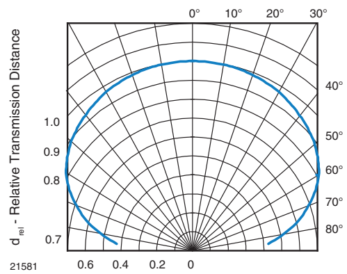
Fig. 11 - Horizontal Directivity
