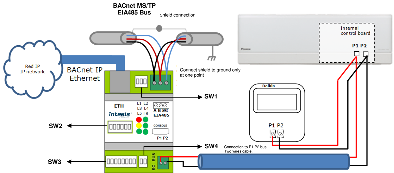
Connection diagram
