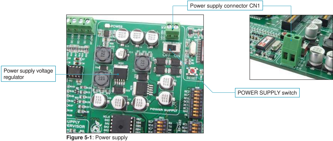
Figure 5-1: Power supply
