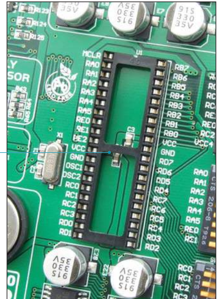
Figure 2-2: DIP40 socket
