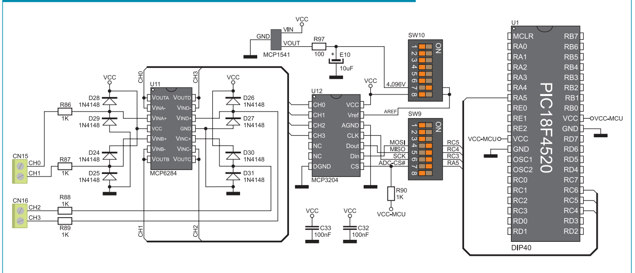
Figure 10-2: AD module and microcontroller connection schematic
