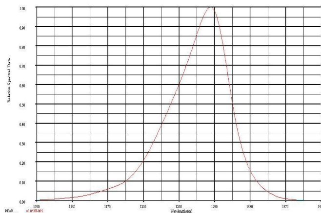
SPECTRAL OUTPUT
