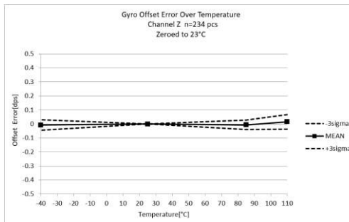
Chart 5 Gyro Offset Error over temperature Z-axis
