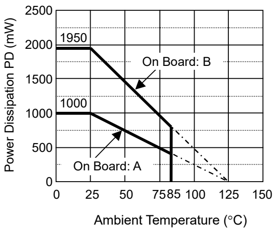
Power Dissipation
