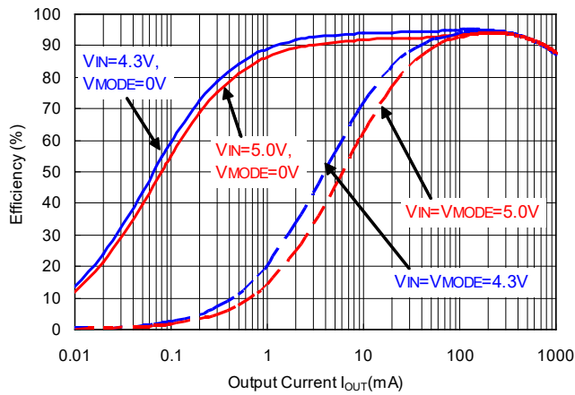
RP550K001A V_{OUT}=3.3V
