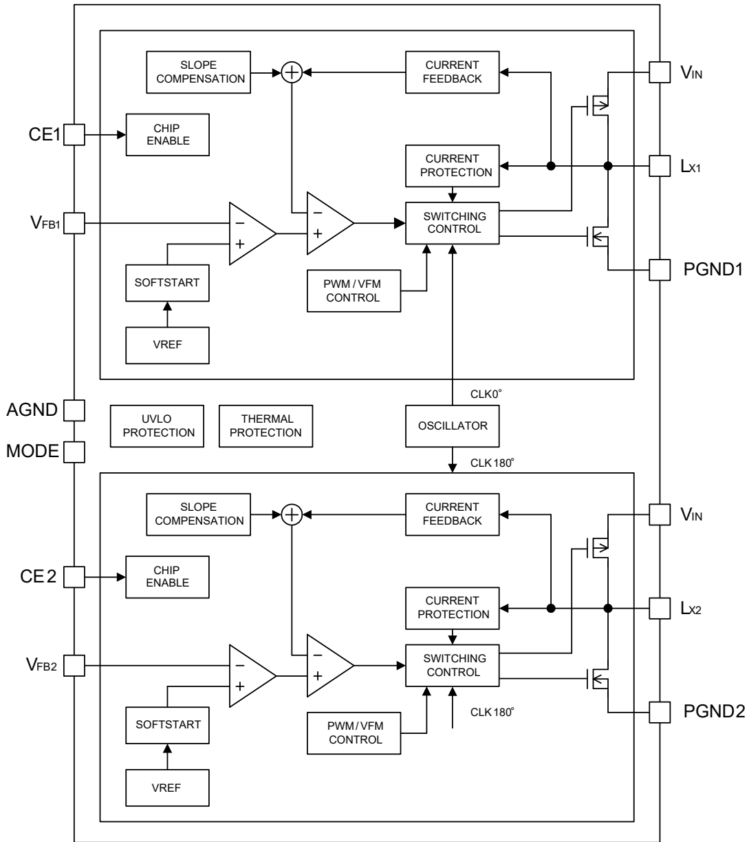
Figure 1. RP550K001A
