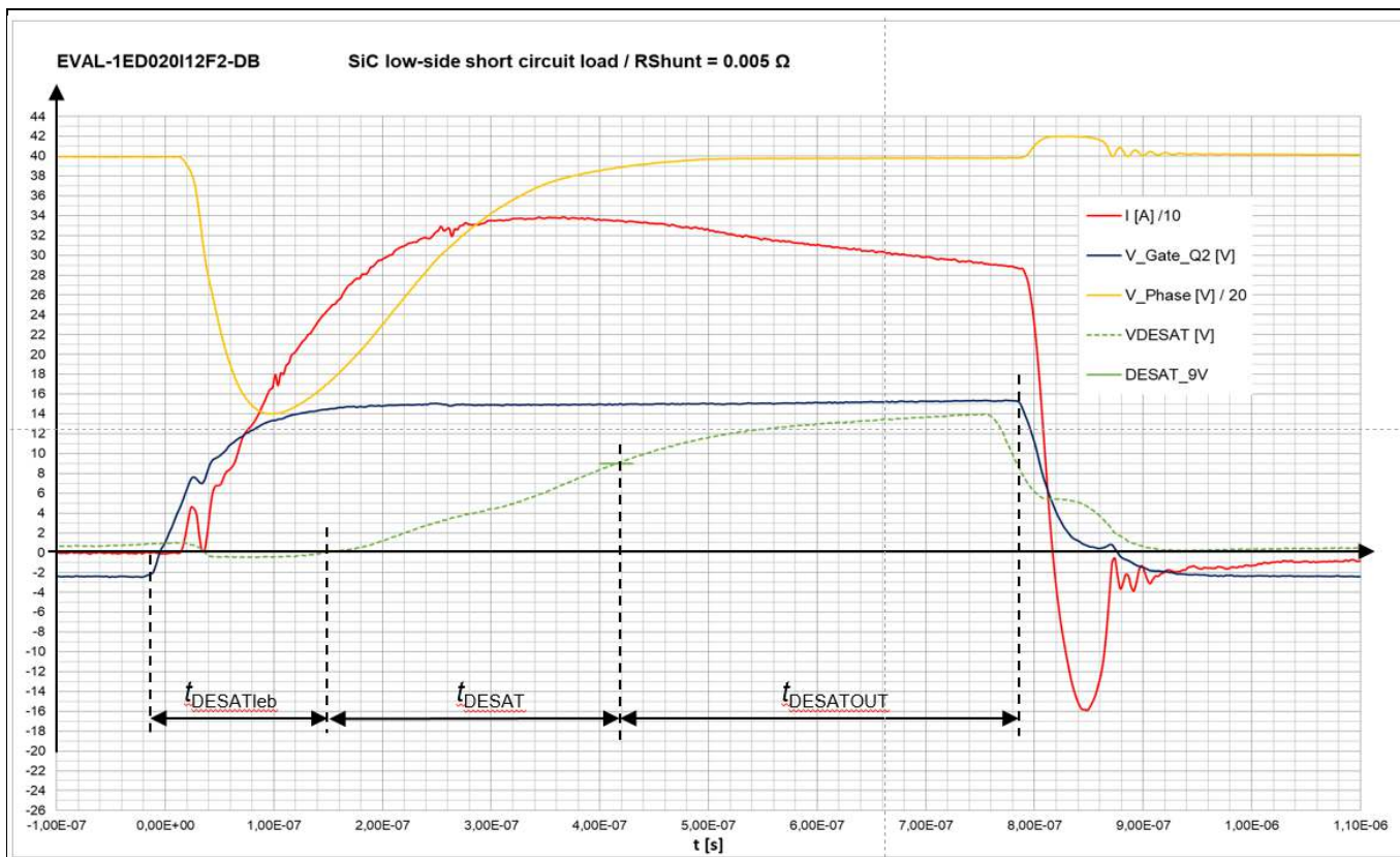
Figure 16 Short circuit measurement at low-side configuration
