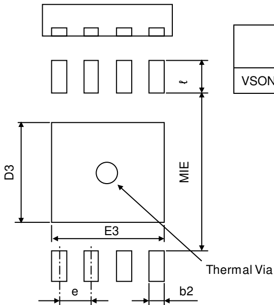
VSON008X2030
