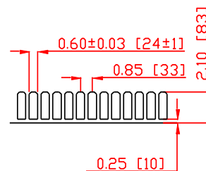
Detail B
