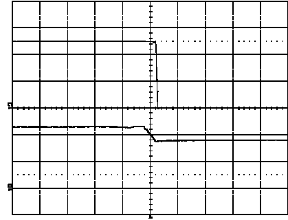
Shut-down enabled by disconnecting V_i at: T_{ref} = +25^\circ\text{C} , I_O = 6\text{ A} resistive load, V_i = 12.0\text{ V} . Top trace: output voltage (2.0 V/div.). Bottom trace: input voltage (5 V/div.). Time scale: 2.0 ms/div.
