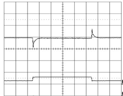
Output voltage response to load current step- Top trace: output voltage (100mV/div.). change (3-6-3 A) at: T_{ref} = +25^\circ\text{C} , V_i = 12.0\text{ V} . Bottom trace: load current (10 A/div.). Time scale: 0.1 ms/div.
