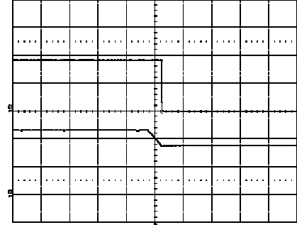
Shut-down enabled by disconnecting V_i at: T_{ref} = +25^\circ\text{C} , I_O = 6\text{ A} resistive load, V_i = 12.0\text{ V} . Top trace: output voltage (1.0 V/div.). Bottom trace: input voltage (5 V/div.). Time scale: 5.0 ms/div.
