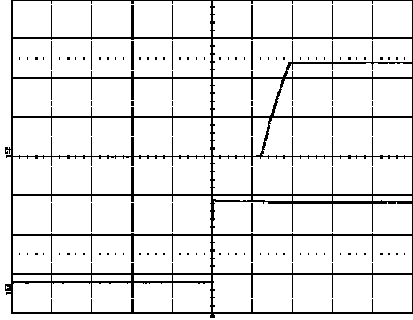
Start-up enabled by connecting V_i at: T_{ref} = +25^\circ\text{C} , I_O = 6\text{ A} resistive load, V_i = 12.0\text{ V} . Top trace: output voltage (2.0 V/div.). Bottom trace: input voltage (5 V/div.). Time scale: 10 ms/div.
