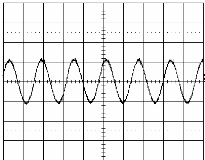
Output voltage ripple (20mV/div.) at: T_{ref} = +25^{\circ}\text{C} , I_O = 6\text{ A} resistive load, V_I = 12.0\text{ V} . Time scale: 2 \mu\text{s}/\text{div} . See the filter in the Output ripple and noise section (EMC Specification).
