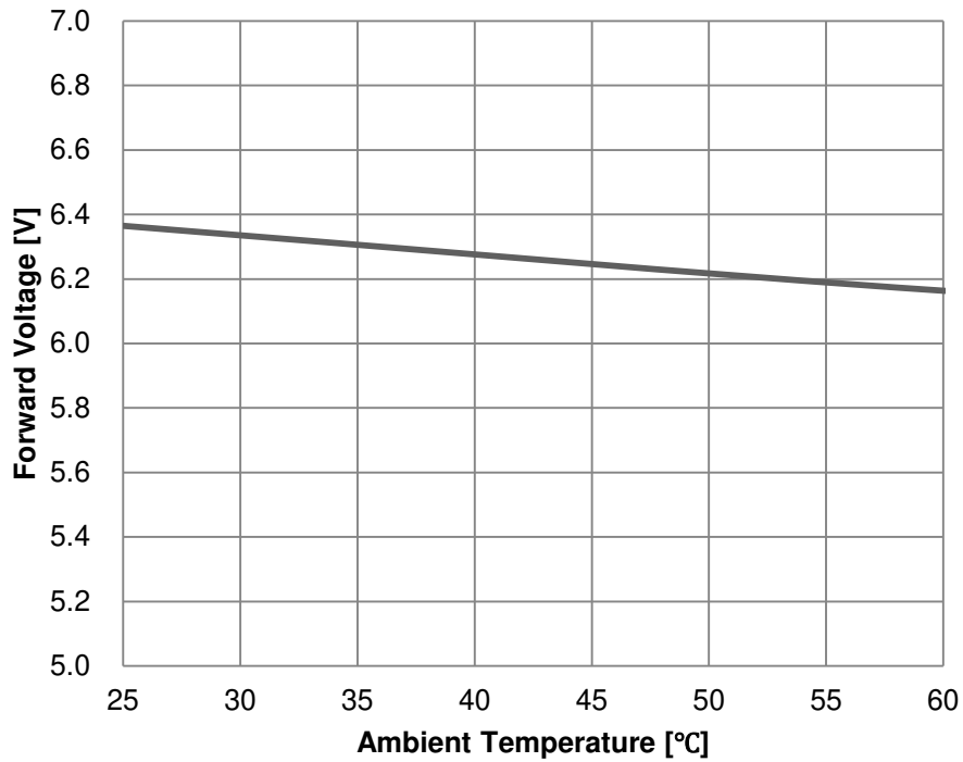
Fig 7. Forward Voltage vs Ambient Temperature, I_F=150\text{mA}
