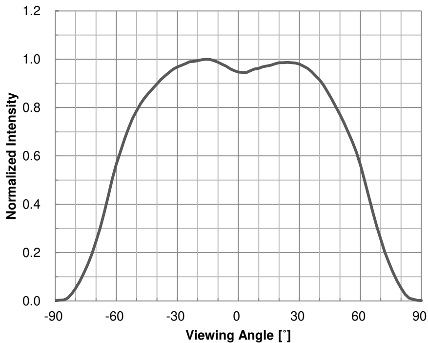
Fig 8. Typical Spatial Distribution, I_F=150\text{mA}
