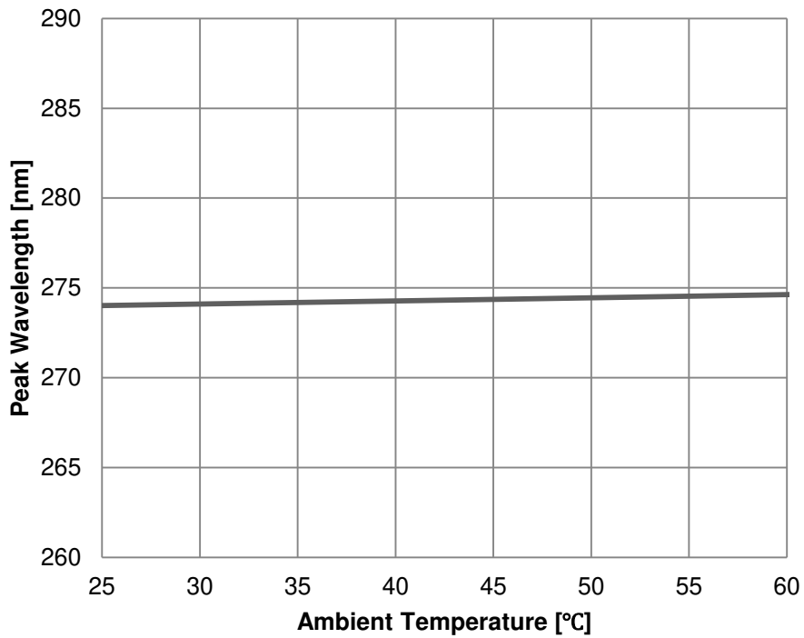
Fig 6. Peak Wavelength vs. Ambient Temperature, I_F=150\text{mA}
