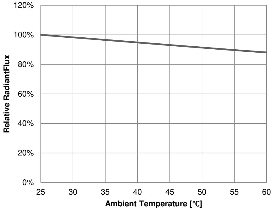
Fig 5. Relative Optical Output Power vs. Ambient Temperature, I_F=150\text{mA}
