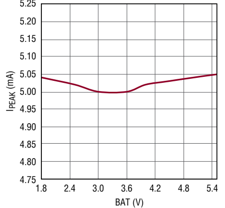
I_{PEAK} vs BAT, 5mA Setting
