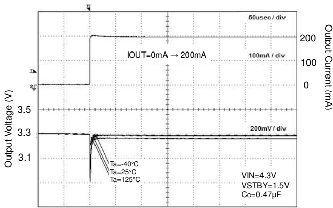
Figure 19. Load Response
