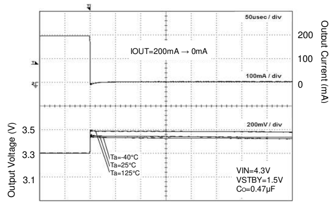
Figure 20. Load Response
