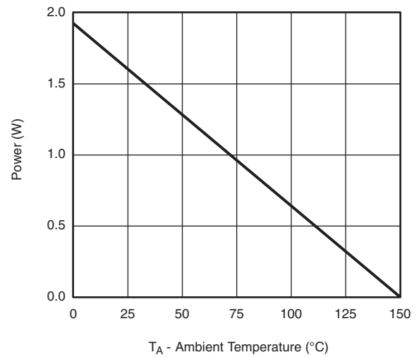
Power, Junction-to-Ambient
