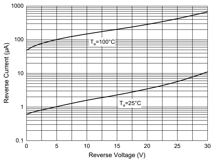
Fig. 2 - Reverse Characteristics
