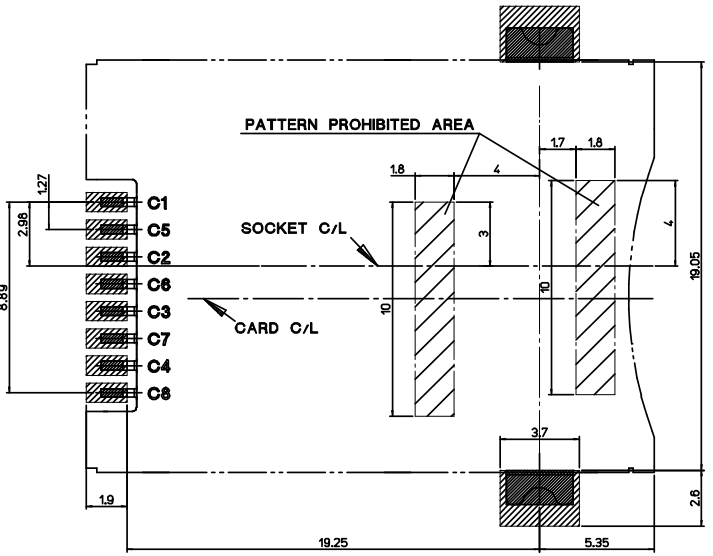
RECOMMENDED PCB PATTERN LAYOUT TOLERANCE : ±0.05
